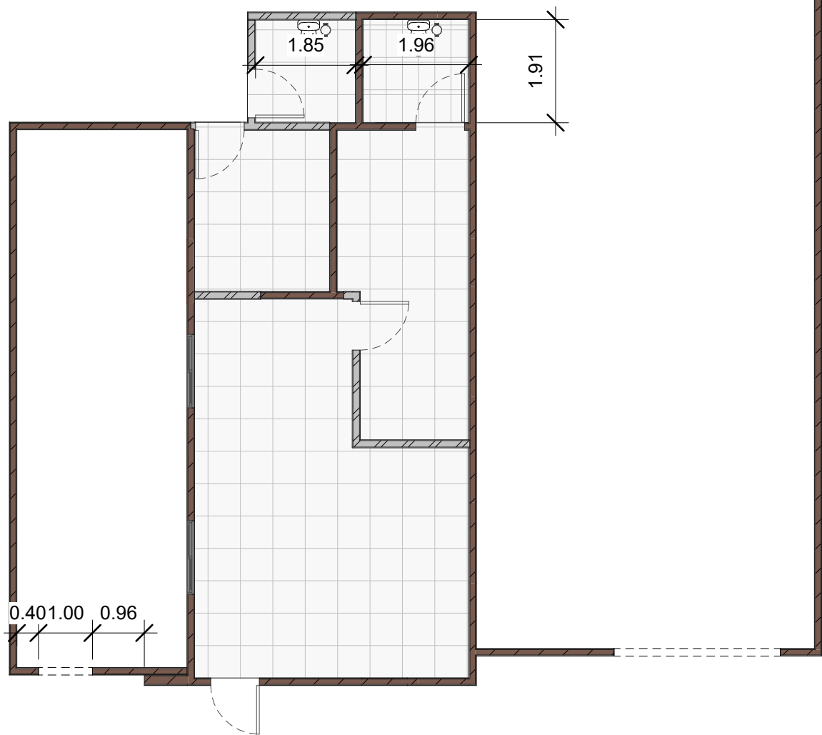
1 AS BUILT 1 : 100
